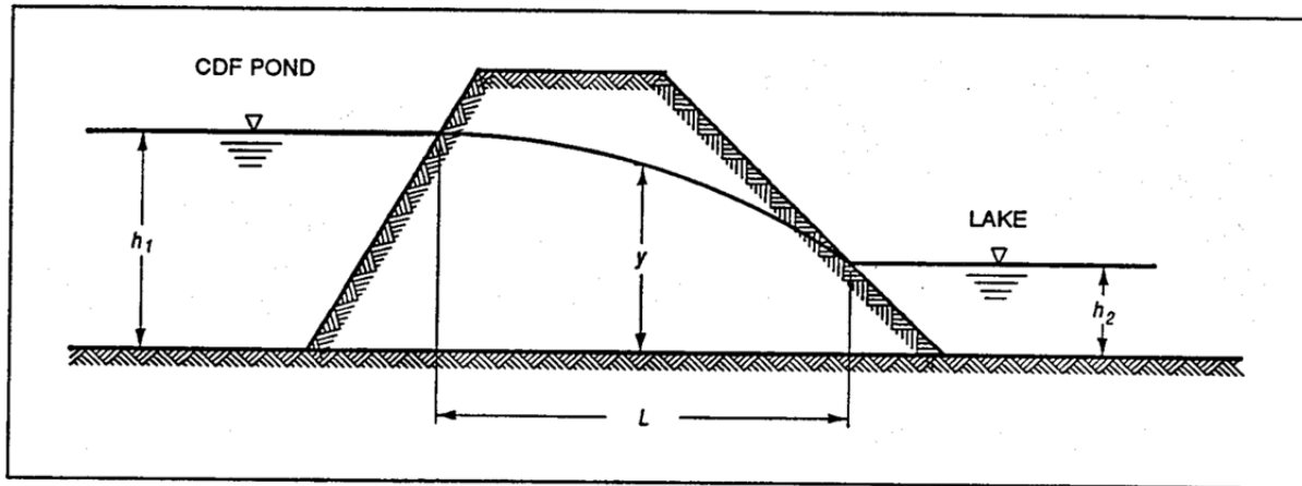
Figure 6. Definition Sketch for Dupuit's Equation (USEPA 1996).
